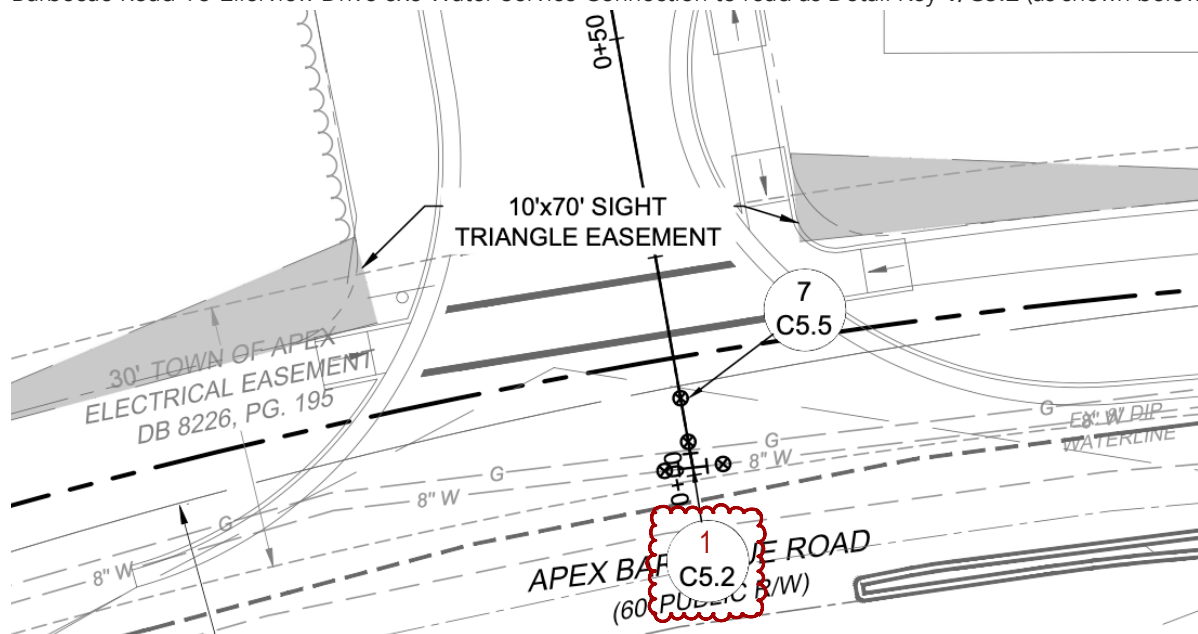
Excerpt from Drawing C3.1 – Utility Plan (Revision 4, Dated 09/25/23)
